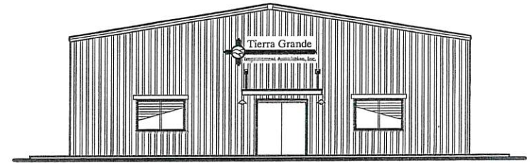
PRELIMINARY NORTH ELEVATION 3/16"-1'-0"
