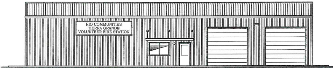
PRELIMINARY WEST ELEVATION 3/16"-1'-0"
