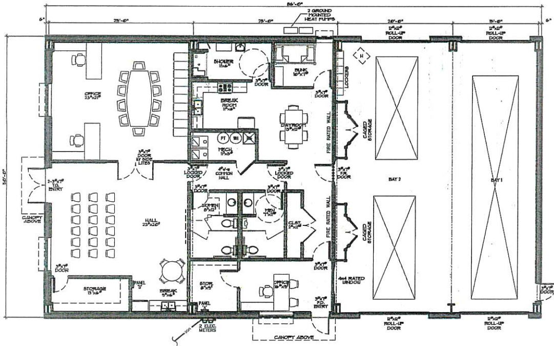
PRELIMINARY FLOOR PLAN OPTION 2 3/16"-1'-0"
